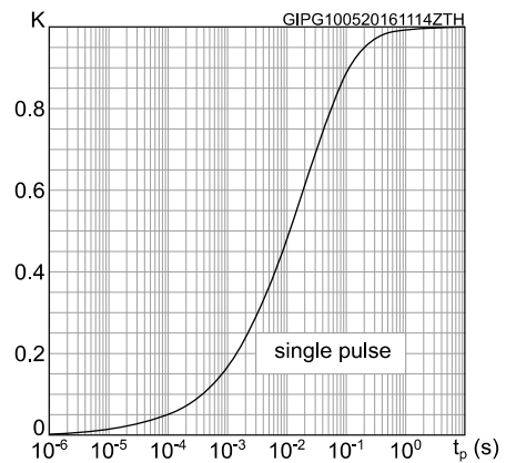
Figure 3: Thermal impedance
