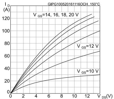
Figure 5: Output characteristics ( T_J = 150^\circ C )
