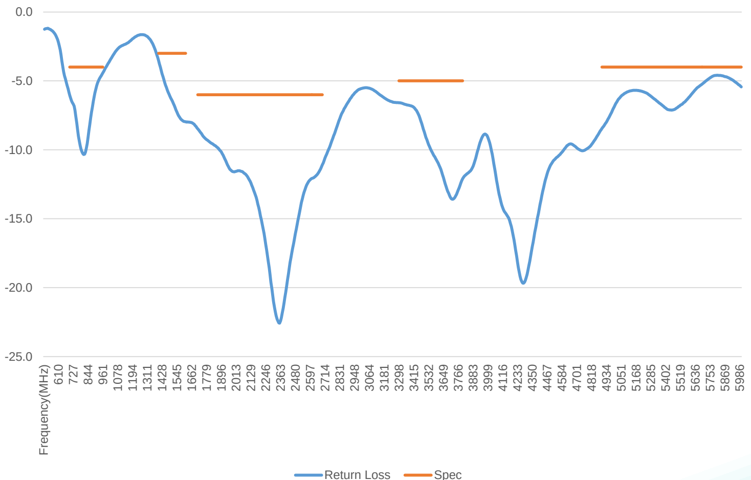
Return Loss
