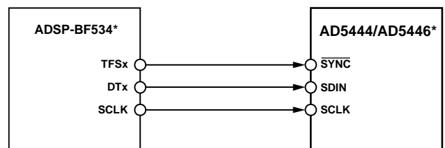
Figure 48. ADSP-BF534 to AD5444/AD5446 Interface
