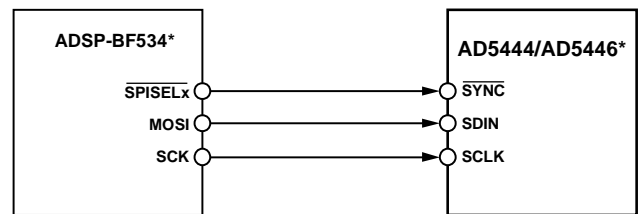
Figure 47. ADSP-BF534 to AD5444/AD5446 Interface
