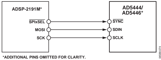
*ADDITIONAL PINS OMITTED FOR CLARITY. 04588-074 Figure 45. ADSP-2191M SPI to AD5444/AD5446 Interface
