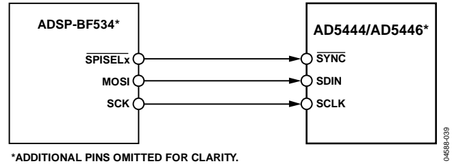
*ADDITIONAL PINS OMITTED FOR CLARITY. 04588-039 Figure 47. ADSP-BF534 to AD5444/AD5446 Interface
