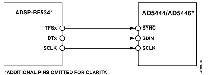
*ADDITIONAL PINS OMITTED FOR CLARITY. 04588-040 Figure 48. ADSP-BF534 to AD5444/AD5446 Interface
