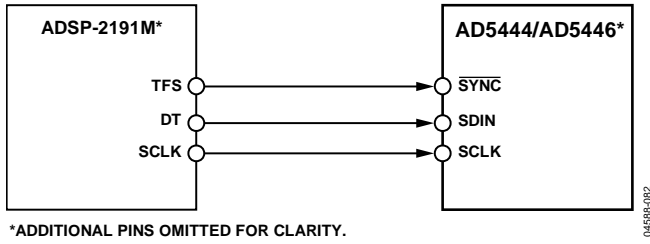
*ADDITIONAL PINS OMITTED FOR CLARITY. 04588-082 Figure 46. ADSP-2191M to AD5444/AD5446 Interface
