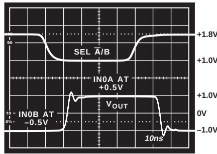
Figure 31. AD8185 Channel-to-Channel Switching Time
