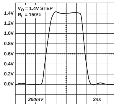
Figure 37. AD8185 Video Amplitude Pulse Response; R_L = 150\ \Omega
