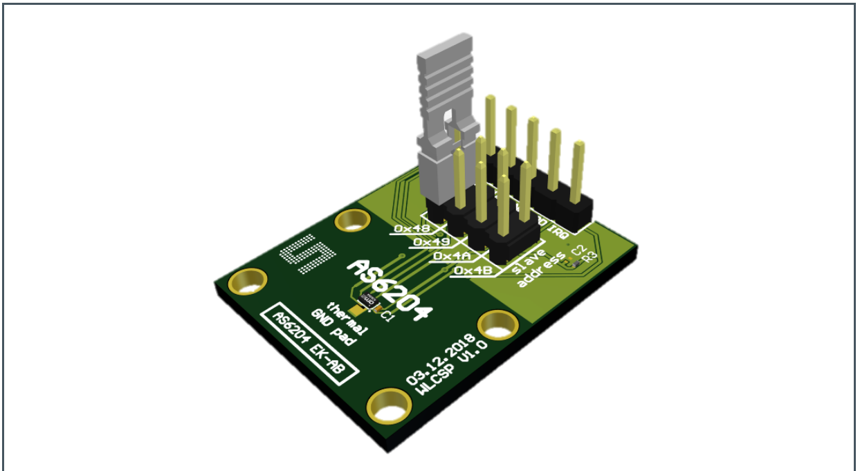
Figure 3: Adapter Board
