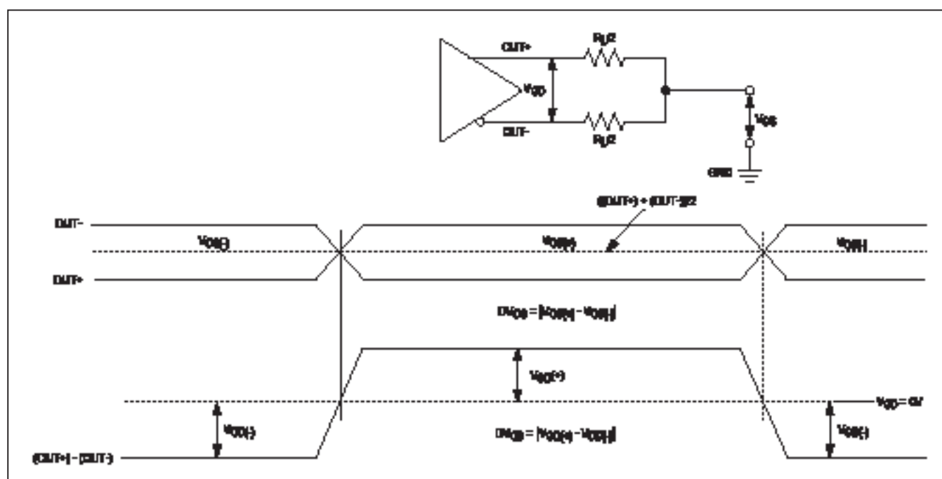
Figure 1. Serial-Output Parameters
