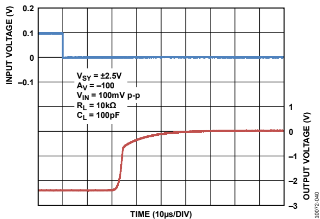
Figure 41. Negative Overload Recovery
