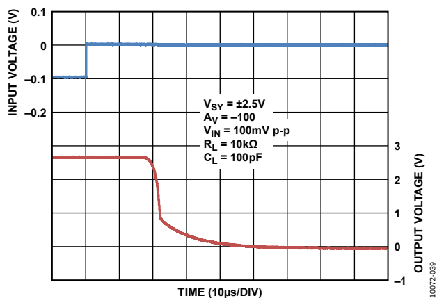
Figure 40. Positive Overload Recovery
