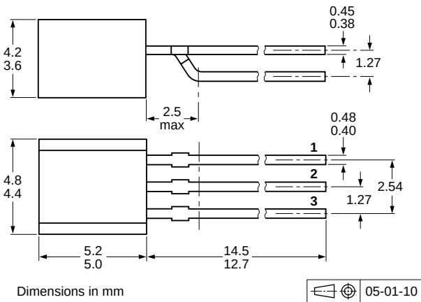
Fig 8. Package outline SOT54 variant
