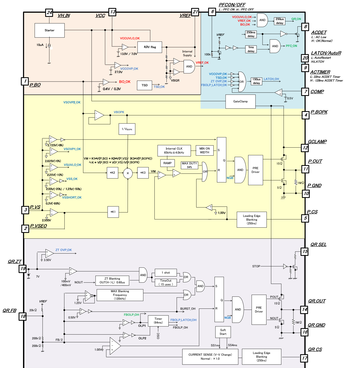
Figure 3-2. Block Diagram
