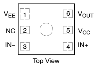
Figure 3. UDFN 1.2x1.0 (NCS2200A)
