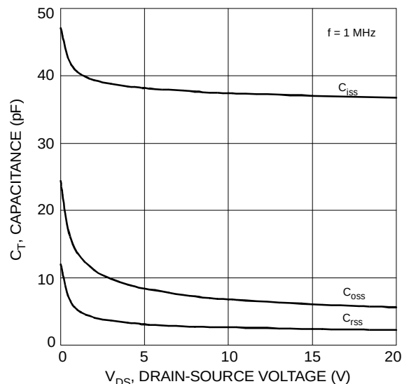
Fig. 10 Typical Capacitance
