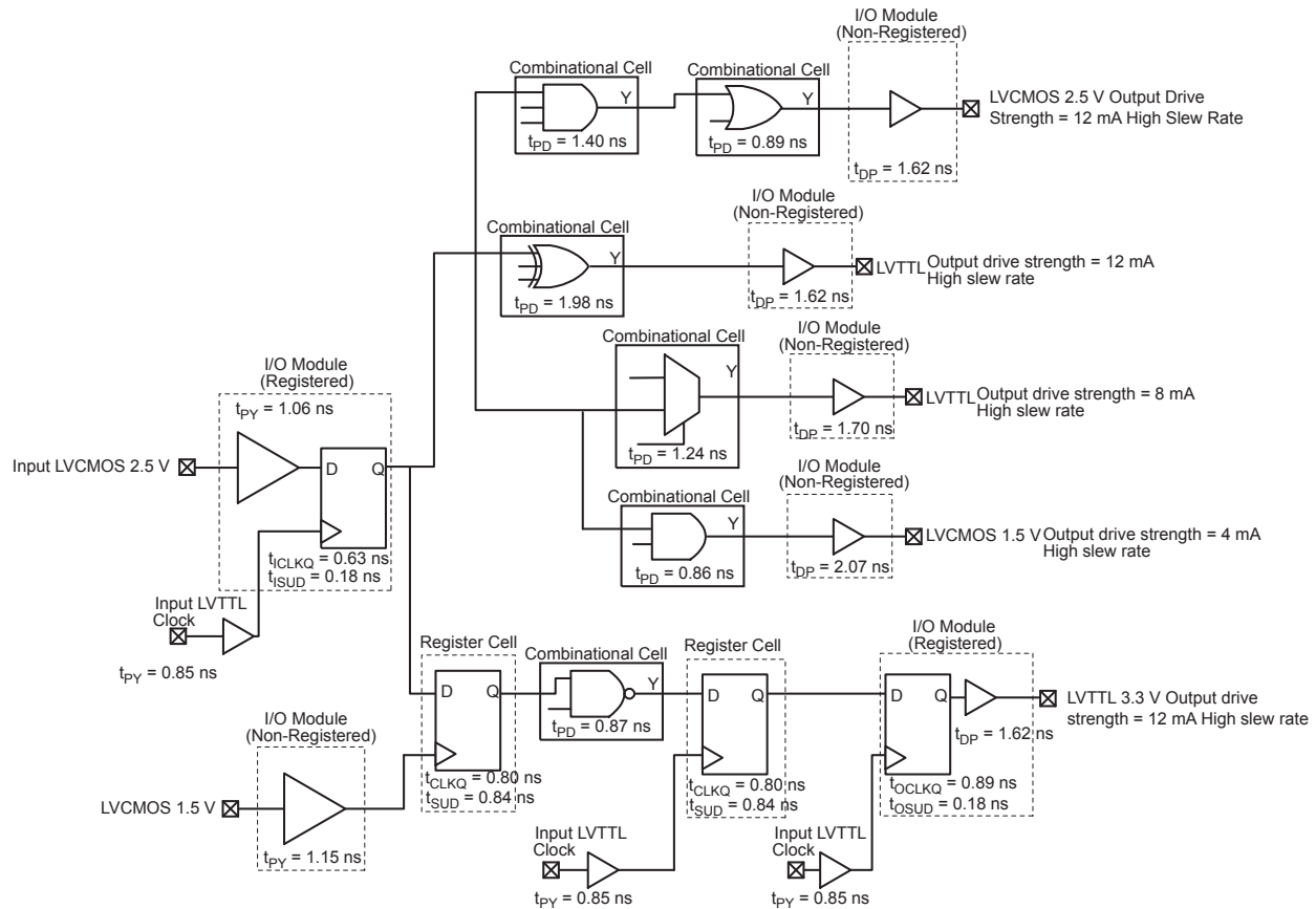
Operating Conditions: STD Speed, Commercial Temperature Range ( T_J = 70^{\circ}\text{C} ), Worst-Case V_{CC} = 1.425\text{ V} , for DC 1.5 V Core Voltage, Applicable to V2 and V5 Devices
