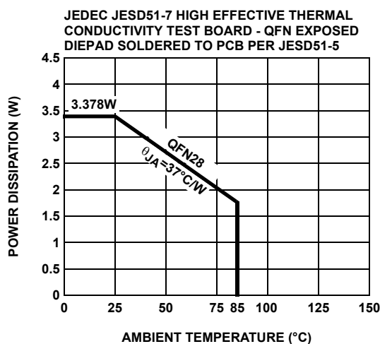
FIGURE 23. PACKAGE POWER DISSIPATION vs AMBIENT TEMPERATURE
