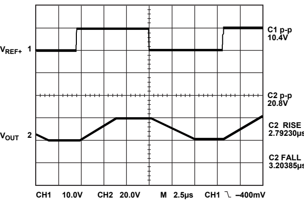
Figure 8. Pulse Response (Large Signal)
