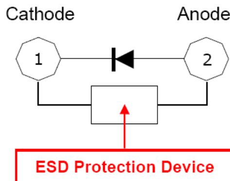
Circuit
