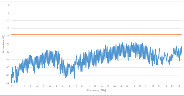
Return Loss SUOFLEX 526S with two straigh PC3.5 connectors
