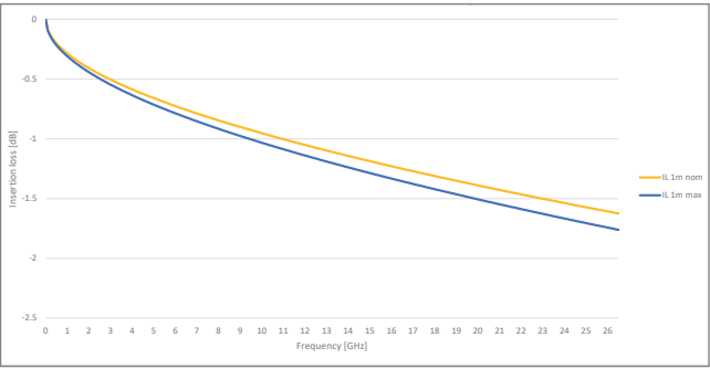
Insertion Loss
