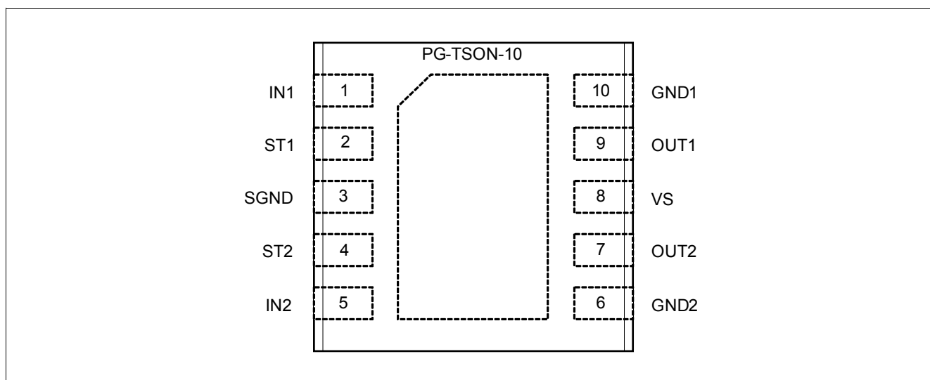
Figure 2 Pin-Out of the ITS42k5D-LD-F
