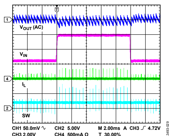
Figure 20. Line Transient, I_{LOAD} = 10\text{ μA}
