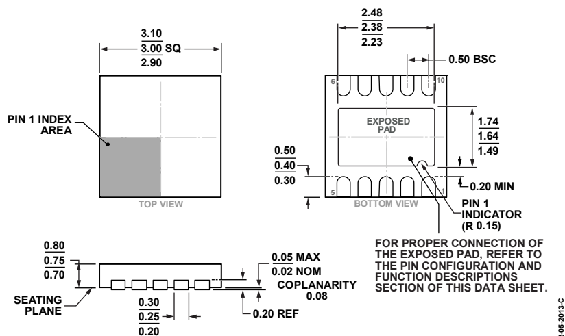
Figure 30. 10-Lead Lead Frame Chip Scale Package [LFCSP_WD] 3 mm x 3 mm Body, Very Very Thin, Dual Lead (CP-10-9)
