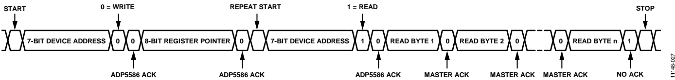
Figure 27. I²C Multibyte Read Sequence
