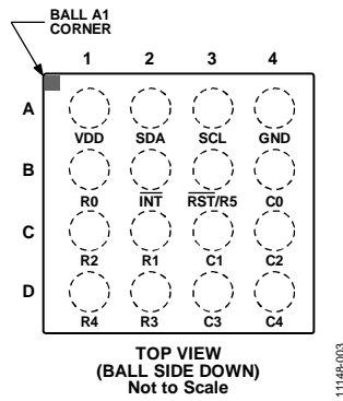
Figure 3. Pin Configuration
