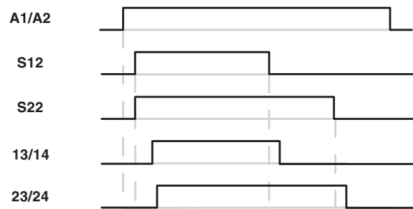
Figure 4 Time diagram
