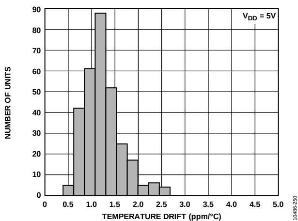
Figure 7. Reference Output Temperature Drift Histogram
