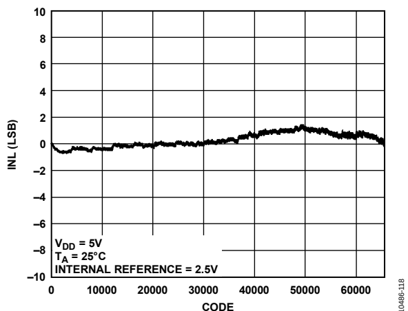
Figure 12. AD5696R INL
