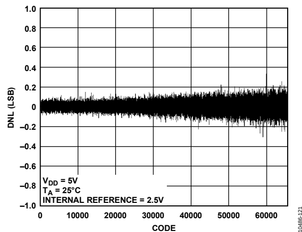
Figure 15. AD5696R DNL
