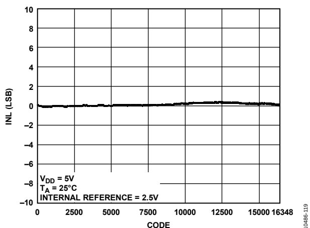
Figure 13. AD5695R INL
