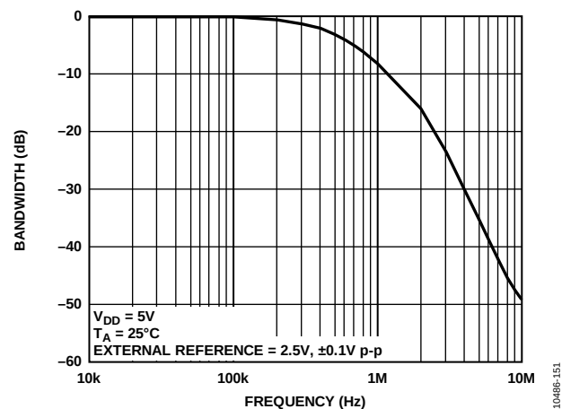
Figure 44. Multiplying Bandwidth, External Reference = 2.5 V, \pm 0.1 V p-p, 10 kHz to 10 MHz
