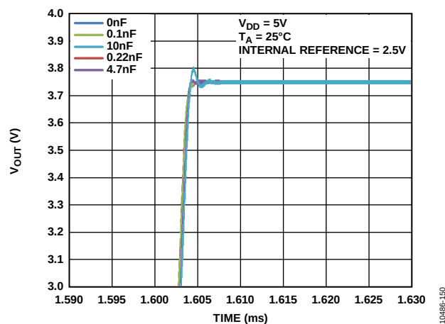
Figure 43. Settling Time vs. Capacitive Load
