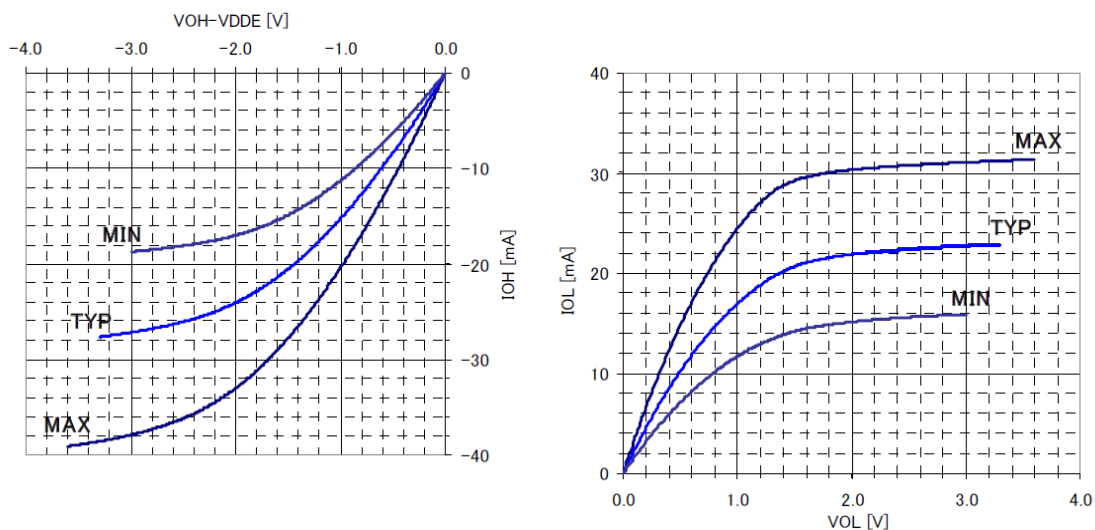
Figure 6-1. V-I curves for pins EINT, AGC0, AGC3
