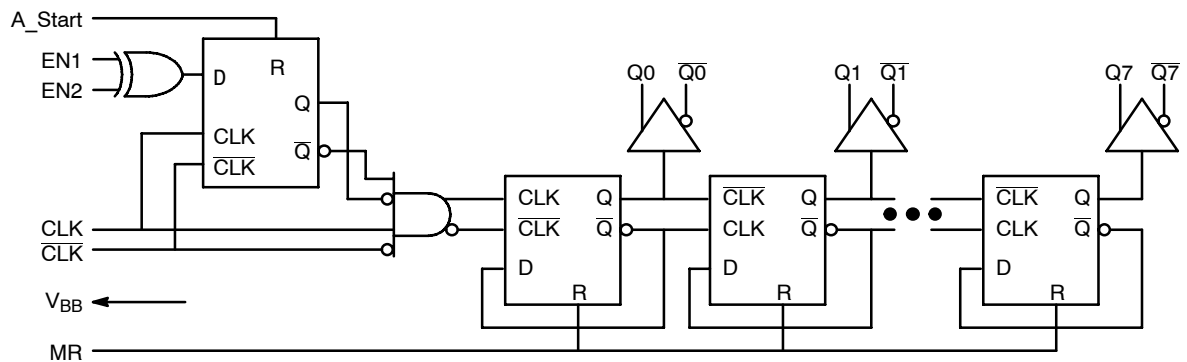
Figure 2. Logic Diagram
