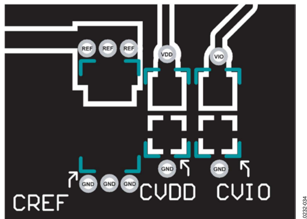
Figure 40. Recommended Layout of the AD7989-1/AD7989-5 (Bottom Layer)
