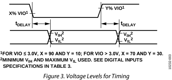
Figure 3. Voltage Levels for Timing
