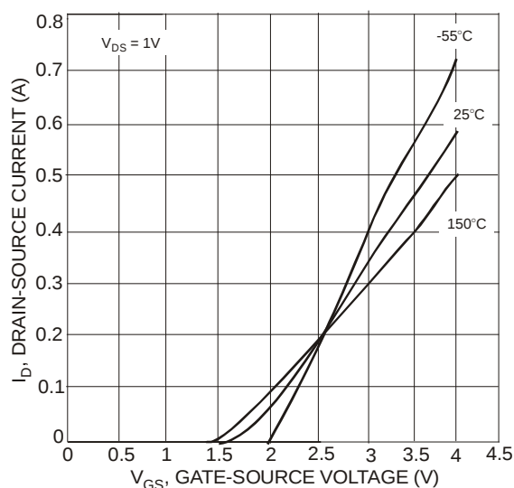
Fig. 2 Transfer Characteristics
