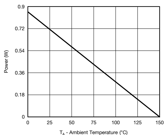
Power Junction-to-Ambient
