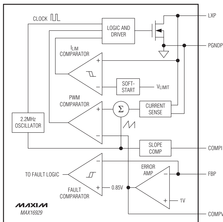
Figure 1. Boost Converter Functional Diagram
