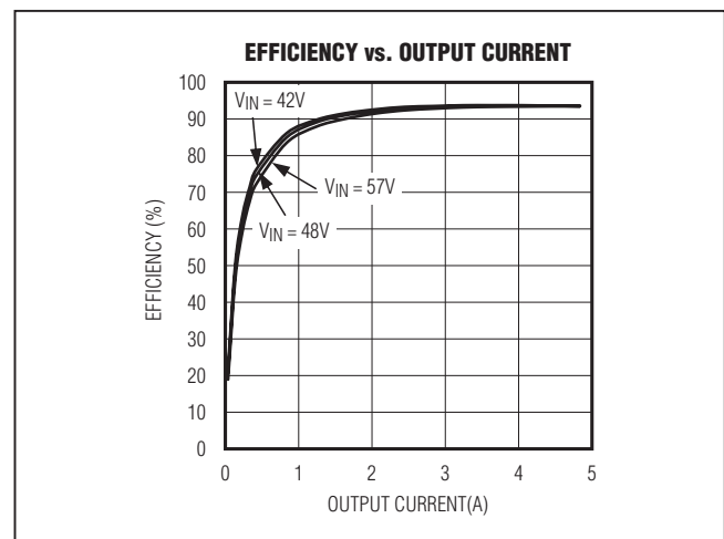
Figure 1. MAX5974C EV Kit Efficiency vs. Output Current at V_{IN} = 42V, 48V, \text{ and } 57V
