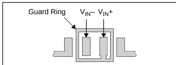
FIGURE 4-11: Example Guard Ring Layout.
