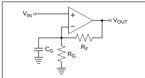
FIGURE 4-5: Non-inverting Gain Circuit with Parasitic Capacitance.
