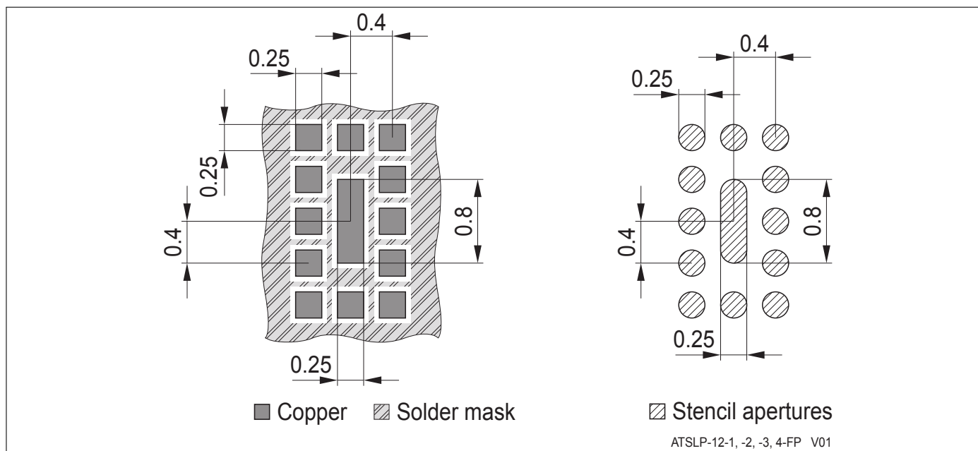
Figure 11: Footprint Recommendation
