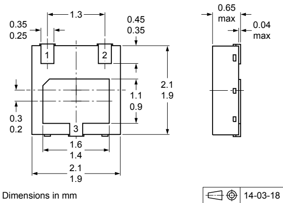
Fig. 15. Package outline DFN2020D-3 (SOT1061D)
