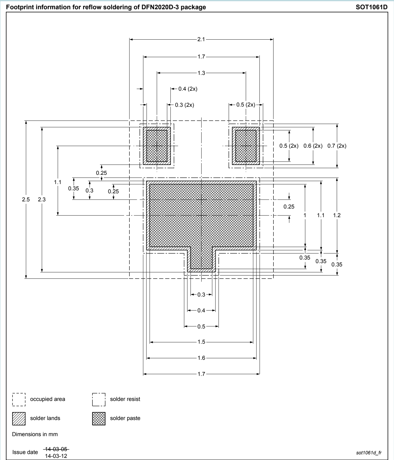
Fig. 16. Reflow soldering footprint for DFN2020D-3 (SOT1061D)
