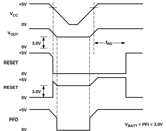
Figure 8. Timing Diagram
