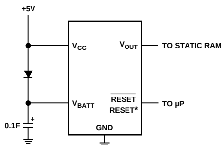
Figure 12. High Capacity Capacitor
