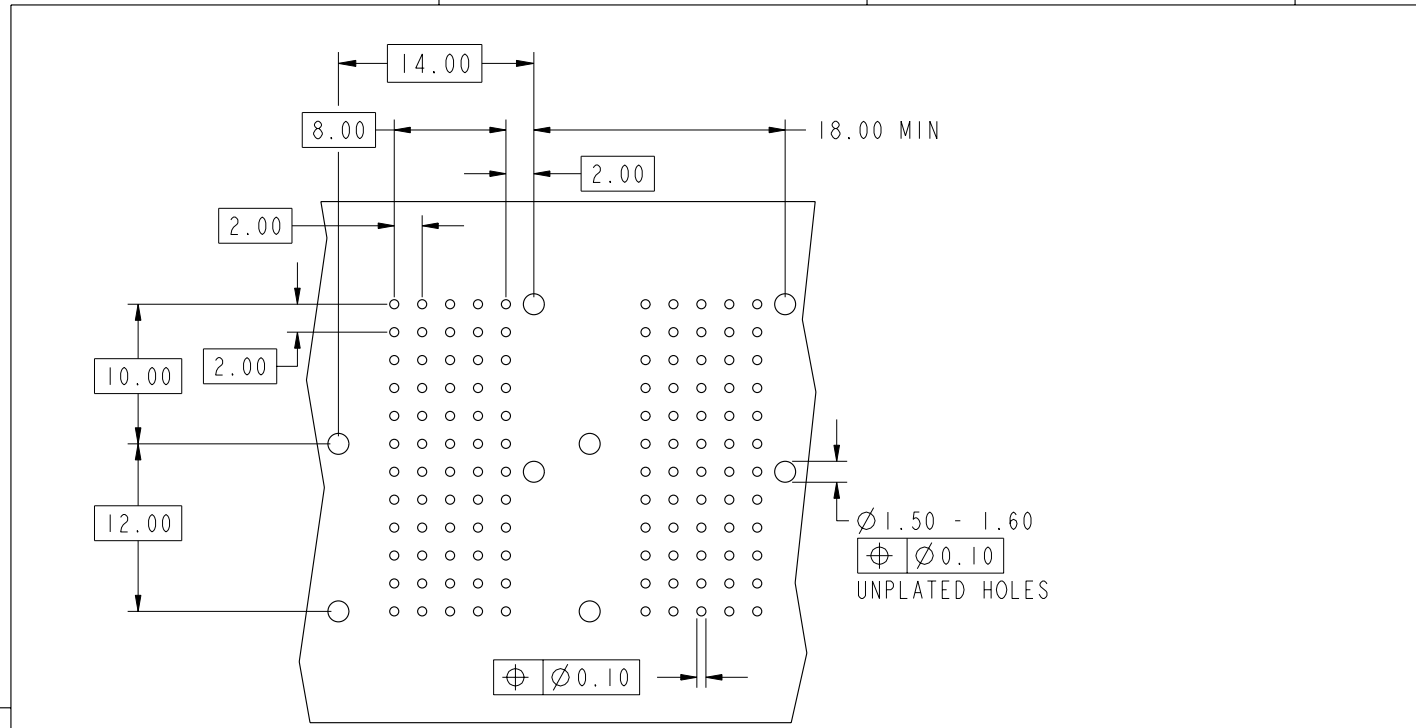
REQUIRED PC BOARD LAYOUT COMPONENT SIDE
