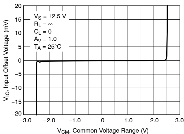
Figure 27. Input Offset Voltage versus Common Mode Input Voltage Range, V_S = \pm 2.5\text{ V}
