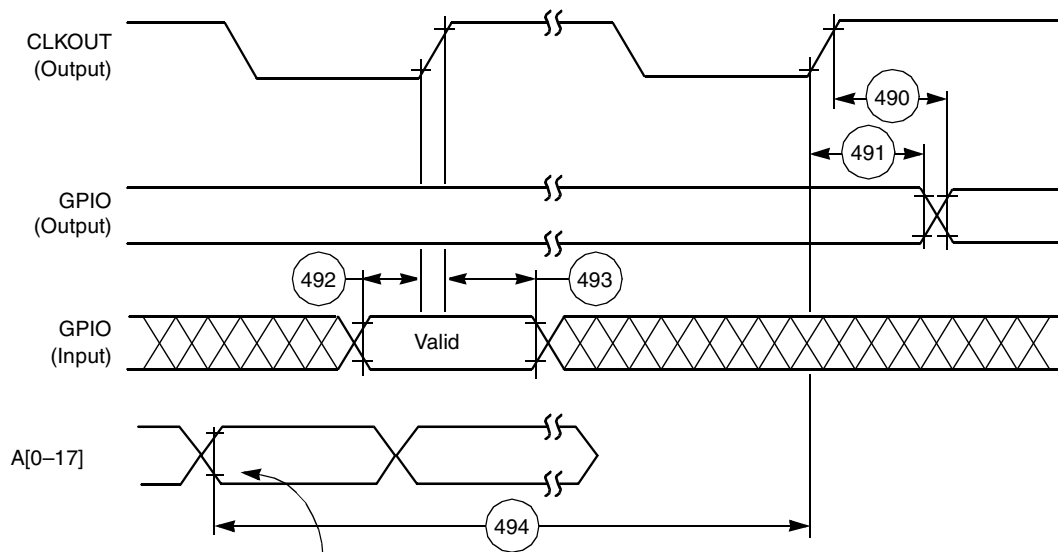
Figure 2-43. GPIO Timing
