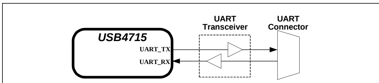
FIGURE 4-5: UART CONNECTIONS
