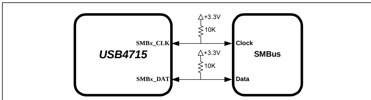
FIGURE 4-3: SMBUS CONNECTIONS
