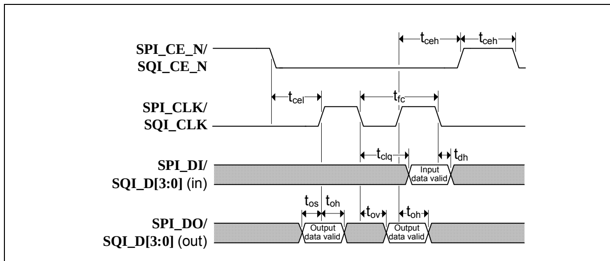
FIGURE 9-5: SPI/SQI TIMING
