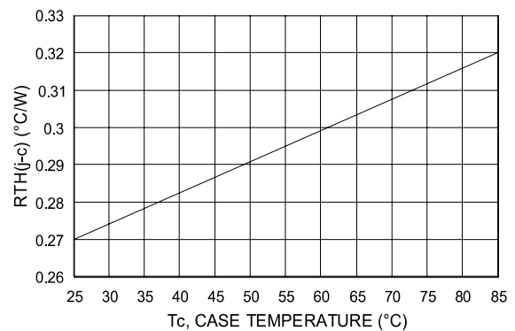
Figure 6: Maximum thermal resistance vs. case temperature
