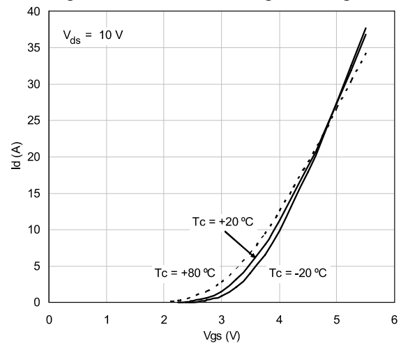
Figure 4: Drain current vs. gate voltage
