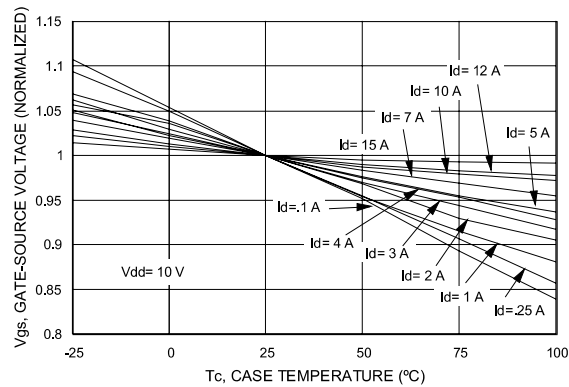
Figure 5: Gate-source voltage vs. case temperature
