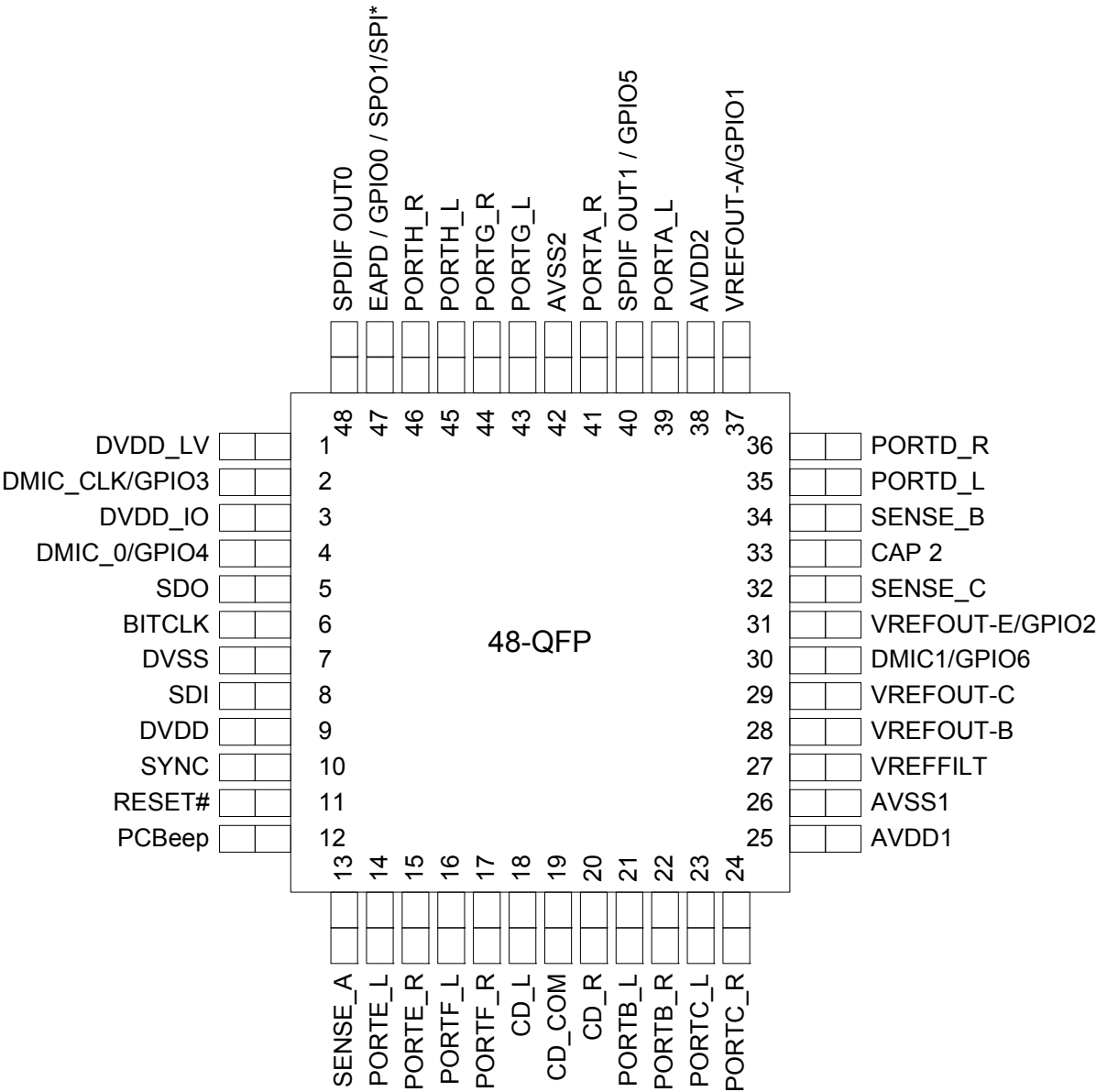
Figure 14. Pin Assignment
