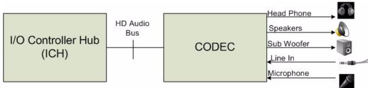
Figure 2. System Diagram
