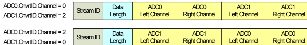
Figure 3. Multi-channel capture
