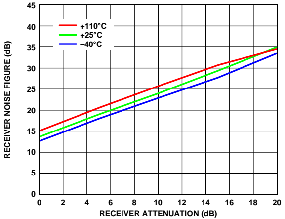
Figure 103. Receiver Noise Figure vs. Receiver Attenuation, LO = 3600 MHz, RF Bandwidth = 200 MHz, Sample Rate = 245.76 MSPS, Integration Bandwidth = 500 kHz to 100 MHz
