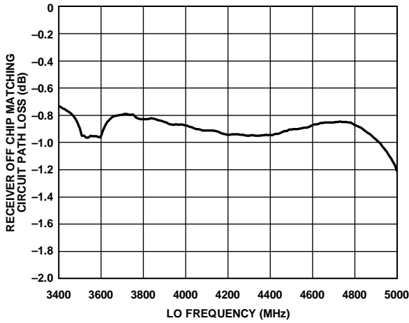
Figure 101. Receiver Off Chip Matching Circuit Path Loss vs. LO Frequency (Simulation), Can Be Used for De-Embedding Performance Data
