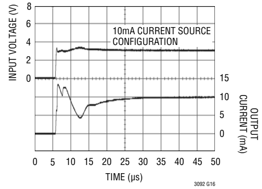
Turn-On Response
