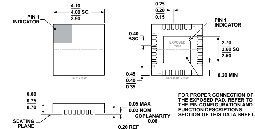
Figure 31. 28-Lead Lead Frame Chip Scale Package [LFCSP_WQ]
