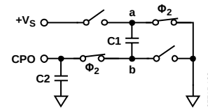
Figure 31. Discharging Cycle
