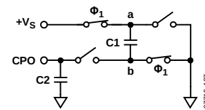
Figure 30. Charging Cycle
