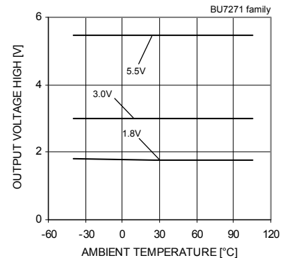
Fig.29 Output Voltage High - Ambient Temperature (RL=10[kΩ])
