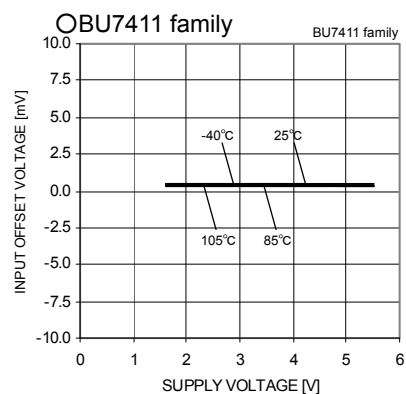
Fig.59 Input Offset Voltage – Supply Voltage ( V_{cm}=V_{DD}-1[V] , V_{OUT}=1.5[V] )
