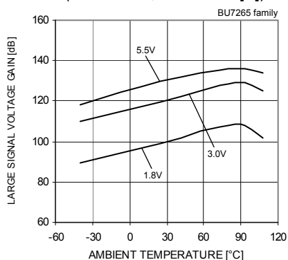
Fig.17 Large Signal Voltage Gain – Ambient Temperature
