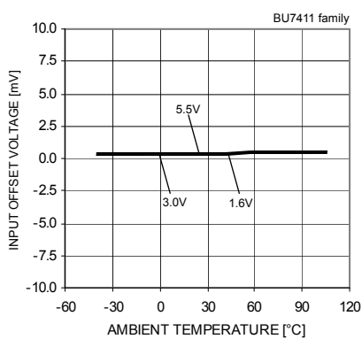
Fig.60 Input Offset Voltage – Ambient Temperature ( V_{cm}=V_{DD}-1[V] , V_{OUT}=1.5[V] )
