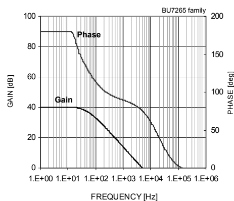
Fig.23 Gain – Frequency
