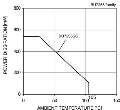
Fig.2 Derating curve
