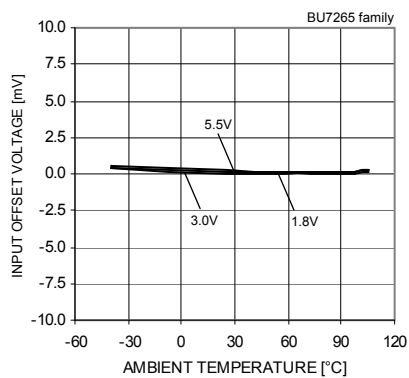
Fig.14 Input Offset Voltage – Ambient Temperature ( V_{icm}=V_{DD} , V_{OUT}=1.5[V] )
