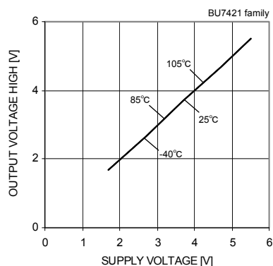
Fig.74 Output Voltage High – Supply Voltage (RL=10[kΩ])
