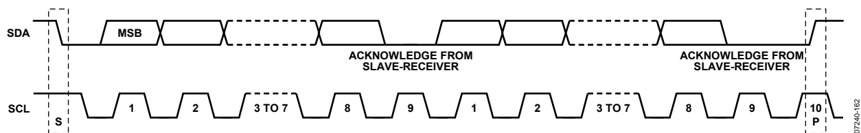
Figure 45. Acknowledge Bit
