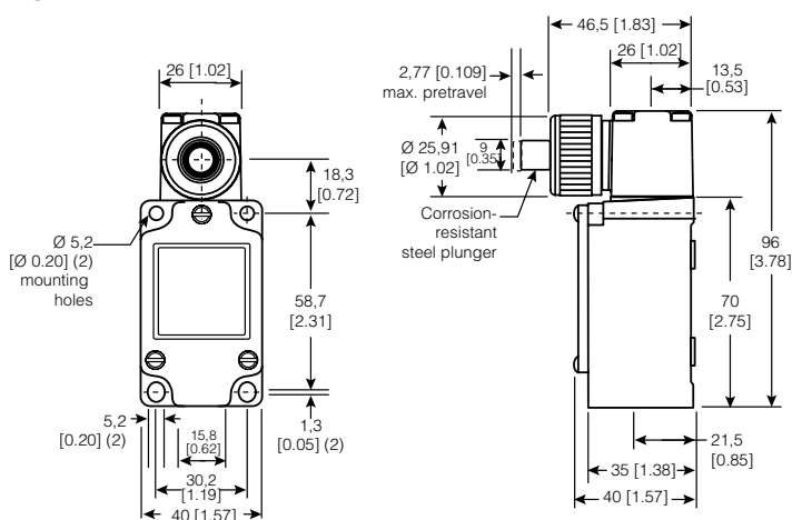
Figure 28. 4LS1-4 Dimensions
