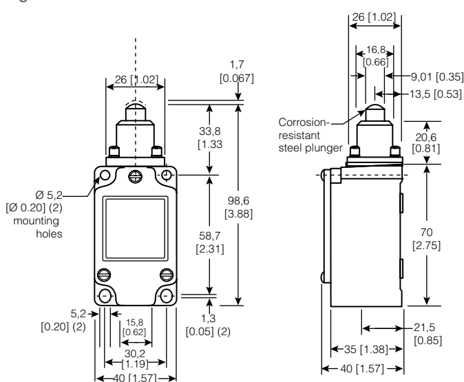
Figure 28. 4LS1-4 Dimensions
