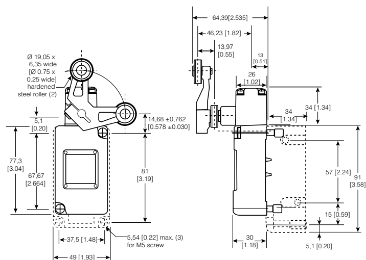
Figure 34. 201LS3-4 Dimensions
