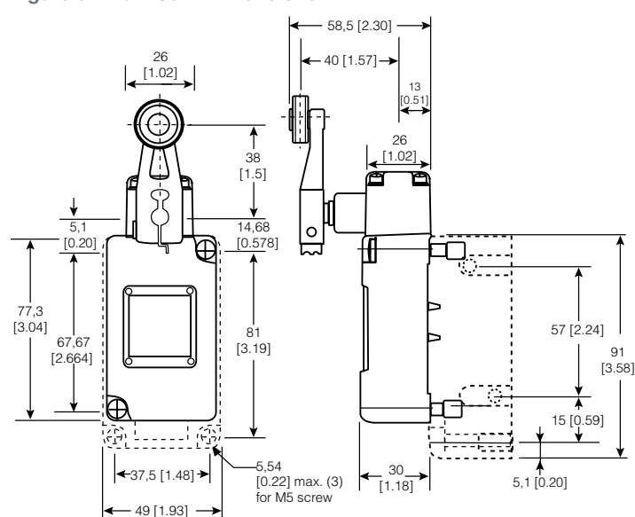
Figure 34. 201LS3-4 Dimensions
