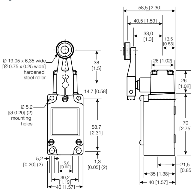
Figure 27. 2LS1-4 Dimensions
