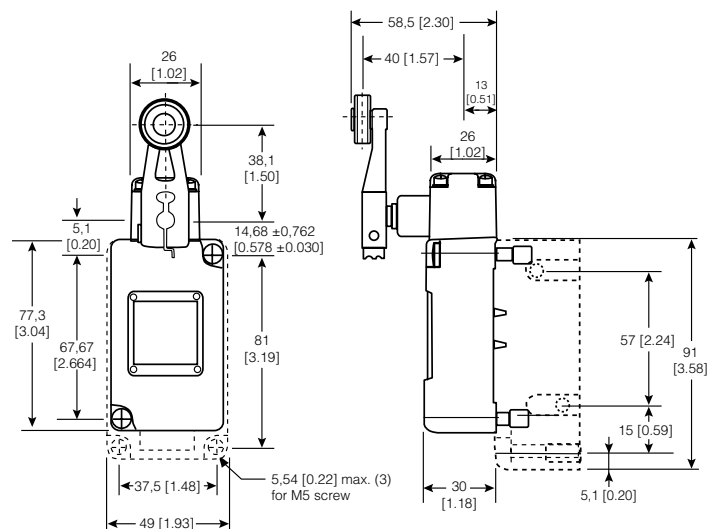
Figure 33. 206LS1-4 Dimensions
