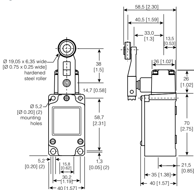
Figure 25. 1LS3-4 Dimensions
