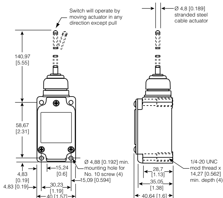
Figure 8. 8LS1 Dimensions
