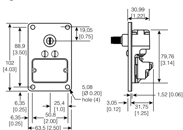
Figure 7. 7LS1 Dimensions
