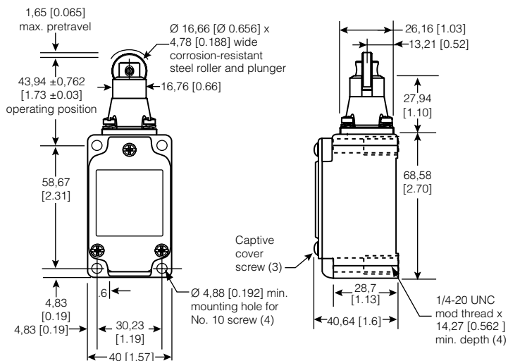
Figure 7. 5LS1 Dimensions
