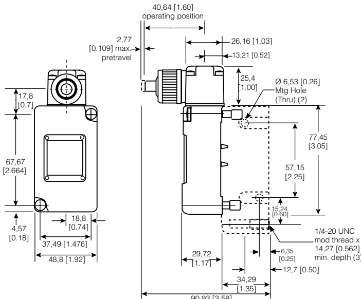
Figure 18. 205LS1 Dimensions
