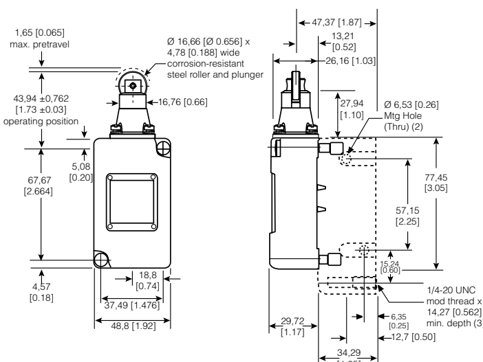
Figure 19. 206LS1 Dimensions
