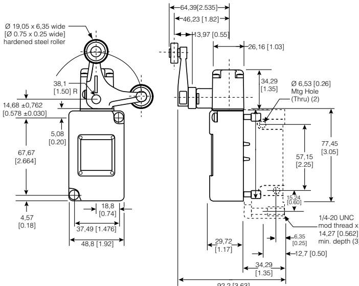
Figure 19. 206LS1 Dimensions
