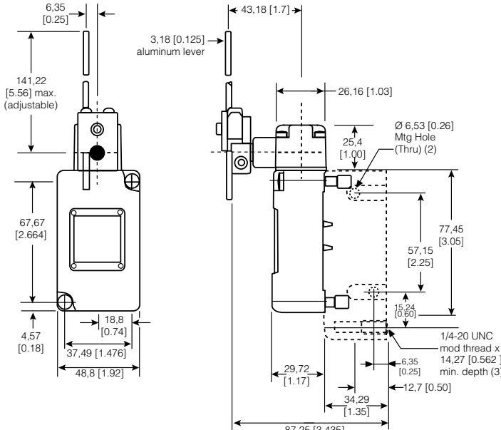
Figure 15. 202LS1 Dimensions
