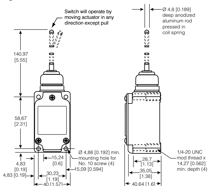
Figure 9. 8LS3 Dimensions
