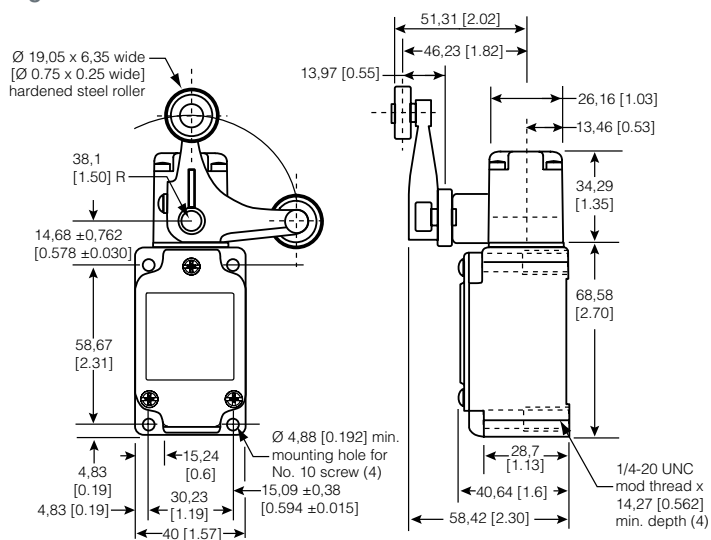
Figure 6. 6LS1 Dimensions
